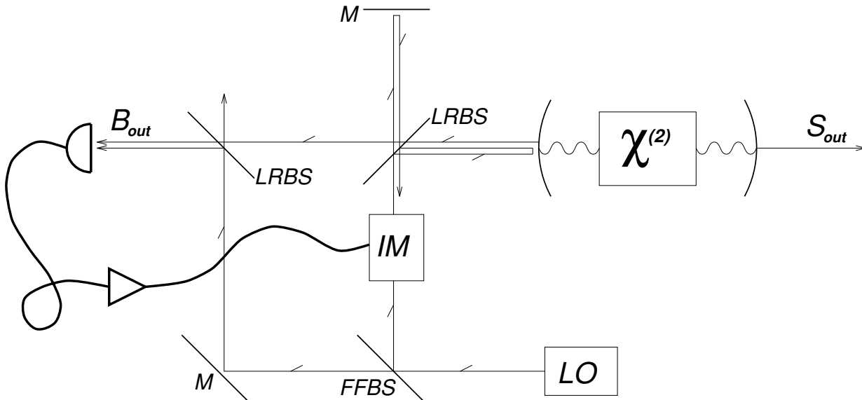
Figure 8.1: Schematic diagram of traveling wave QND device using feedback. The current-carrying wire is indicated by a thick curve; narrow lines represent light beams. S_{out} and B_{out} are the signal and probe output beams, as explained in the text. LO denotes the local oscillator source, IM a current-controlled intensity modulator, M a mirror, LRBS a low reflectivity beam-splitter, and FFBS a 50/50 beam splitter.
